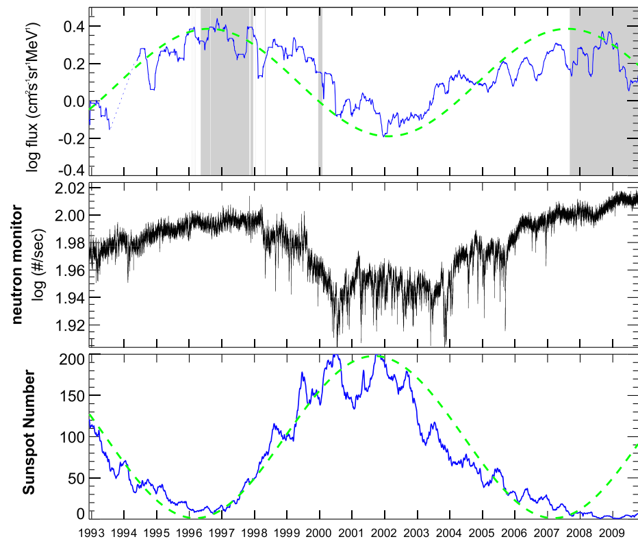
Figure 2. Top panel, long-term measurements of 27.4- to 37.4-MeV proton fluxes at L = 1.33\text{--}1.42 by SAMPEX/PET ( http://www.srl.caltech.edu/sampex/DataCenter/ ) with a 100-day running average. Data points are only kept if they are close to 500 km in altitude (within a 20-km margin). Time periods marked by the gray background are when SAMPEX was spinning and data in these periods are multiplied by a factor of 2 in order to match the fluxes to those in the normal mode when SAMPEX was zenith pointing. Data from 21 September 1993 to 17 March 1994 are not reliable due to the satellite operation and are removed. (2) Daily averaged neutron count rates as measured by the neutron monitor located in Delaware, USA ( L \approx 2.4 ) ( http://neutronm.bartol.udel.edu/ ). Data points with values greater than 105% or less than 95% of the previous 50-day averaged count rate are removed. (3) 100-day running average sunspot numbers. The dashed green curves on top and bottom panels are fitted sine curves with an 11-year period.
