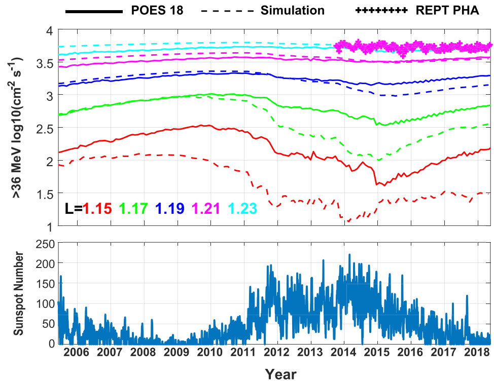
Figure 6. Top panel: omnidirectional integral fluxes of >36-MeV protons mirroring near the magnetic equator with B/B_{\min} < 1.01 for different L (color-coded). Solid lines, from June 2005 to February 2018, are from POES-18 P7–P9 sensor, which are omnidirectional solid-state detectors with 120^\circ FOV for P7 and 180^\circ FOV for P8 and P9 (Evans & Greer, 2004). The geometric factors used to convert the count rate of omnidirectional solid-state detectors to the flux are obtained from appendix F of Evans and Greer (2004). After 2015, only differential fluxes from POES-18 are available, the integral fluxes here are calculated from raw format POES-18 data ( https://satdat.ngdc.noaa.gov/sem/poes/data/raw/ngdc/ ), and a factor of 0.85 is multiplied to the calculated integral fluxes to ensure a smooth transition between the end of 2014 and the start of 2015; dashed lines are for simulation results based on a theoretical model (Selesnick et al., 2007; Selesnick & Albert, 2019); the “+” dots are for Van Allen Probes/REPT PHA data (for L = 1.21 only) from October 2013 to February 2018. Bottom panel: daily averaged sunspot numbers. Due to offset of the Earth’s center and dipole center, POES-18 is able to cross the magnetic equator at different L (up to L = 1.23 ) at different longitudes.
