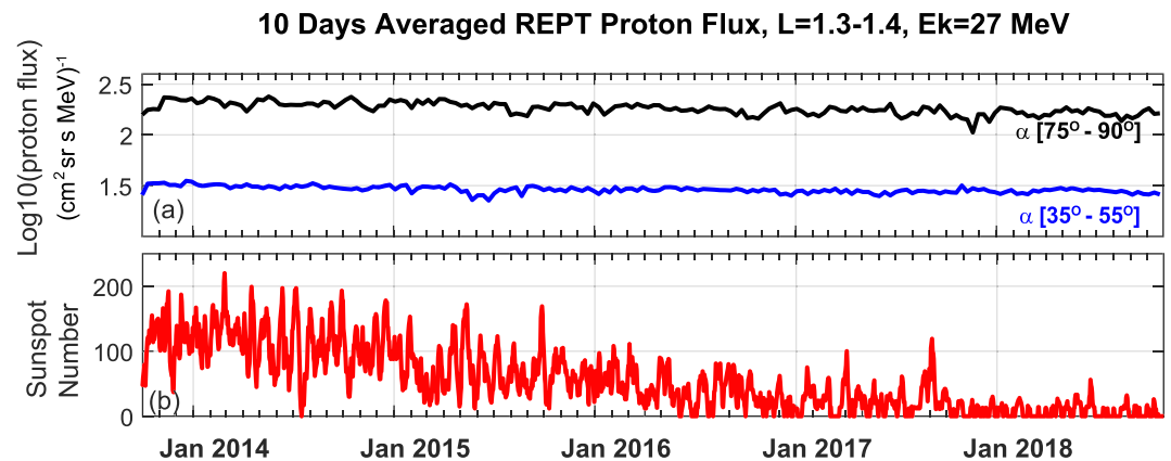
Figure 5. Proton fluxes determined from REPT/PHA data (Selesnick et al., 2014, 2018) measured by Van Allen Probes/REPT are plotted in Panel (a): 10-day averaged 27-MeV proton flux at L = 1.3 – 1.4 during October 2013 to October 2018. The L bin is 0.1, the energy resolution is 4 MeV, and the equatorial pitch angle resolution is 7.2^\circ . The black curve and blue curve present the average proton flux in equatorial pitch angle range 75 – 90^\circ and (35 – 55^\circ , respectively; Panels (b): daily averaged sunspot number.
