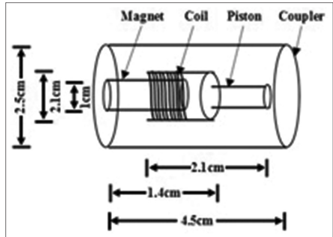
Figure 7: Internal parts of the transducer
