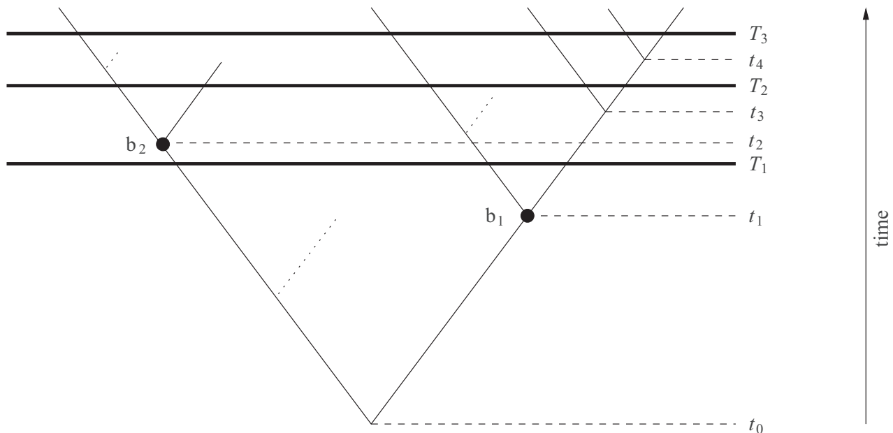
Figure 3. A rooted binary phylogenetic tree with three times T_1, T_2, T_3 at which taxa have been sampled. The dotted branches refer to taxa that do not contribute to the expected distances from one of these times to another and thus are not taken into account. On the other hand, bifurcation b_2 at time t_2 shows that extinction may have an impact on the expected values. Such branches have to be considered.
