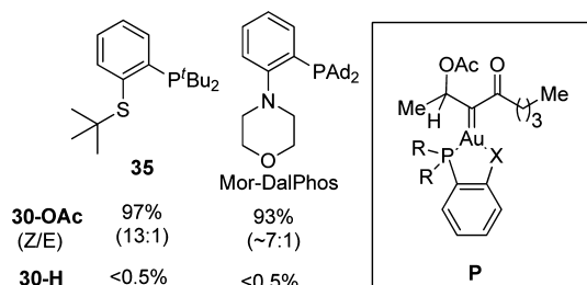
FIGURE 3. The impact of ligands on the ratio of 30-OAc and 30-H in the gold-catalyzed oxidation of 29 (reaction conditions 5 mol % gold catalyst, 1.5 equiv of 8-methylquinoline N -oxide, DCE, rt, 3 h).
