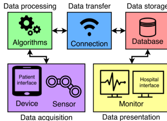
Figure 3. Overview of the processes and corresponding technical components of a telemonitoring system.
