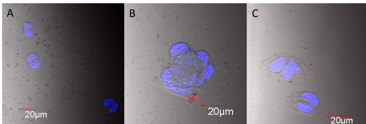
Figure 5 Confocal microscope images of Caco-2 cells stained with DAPI (blue) and treated with QD(A), QD(B) and QD (C). (QDs are red).
