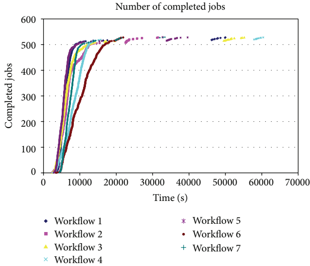
FIGURE 2: Number of completed jobs over time. Each workflow needs to wait for the completion of all its jobs in order to produce the final result. While most of the jobs finish within 10000 seconds, the last ones need much more time to complete. These last jobs almost triple the makespan (from roughly five to fifteen hours).
