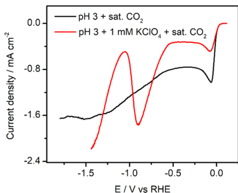
Figure 2. Linear sweep voltammetry of Pd ML Pt(111) in CO 2 -saturated pH 3 electrolytes in the absence (black) and presence of 1 mM KClO 4 (red). Scan rate: 10 mV s -1 .
