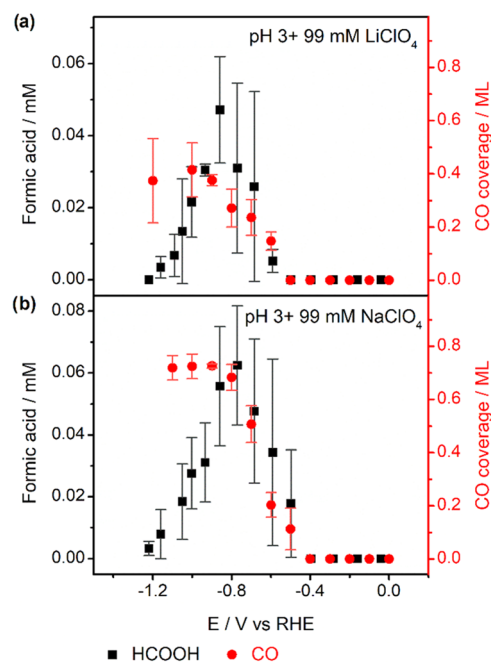
Figure 4. Cation identity effect on \text{Pd}_{\text{ML}}\text{Pt}(111) . \text{CO} coverage and HCOOH formation during \text{CO}_2\text{RR} obtained in \text{CO}_2 -saturated pH 3 electrolytes containing 99 mM (a) \text{LiClO}_4 and (b) \text{NaClO}_4 . Error bars are standard deviations based on three independent measurements.
