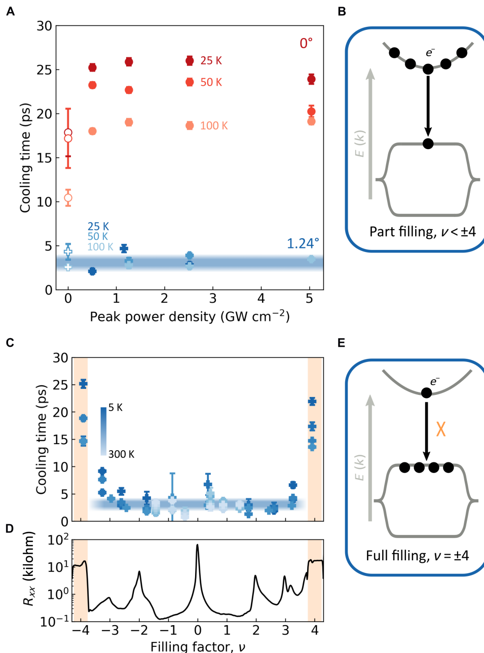
Fig. 3. Origin of enhanced cooling in MATBG. (A) Dependence of cooling time on peak power density for BLG (red circles) and MATBG (blue crosses). The filled (open) shapes are measured using the TrPV (CW-PM) technique. The error bars signify the one sigma confidence interval from the fitting algorithm. (B and E) Schematics of cooling power in MATBG for part filling (B) and full filling (E) of the flat bands. For part filling, the interband transition is not rate-limiting as evidenced by the absence of a power dependence in (A). At full filling, cooling times are longer because of the interband bottleneck effect illustrated in (E). (C and D) Gate dependence of cooling time (C) and four-terminal resistance acquired at T = 35 mK ( R_{xx} ) (D). Orange-shaded region highlights full filling of the moiré unit cell, where R_{xx} and cooling time increase. In (A) and (C), the error bars signify the one sigma confidence interval from the fitting algorithm, and the thick blue line represents the cooling time obtained from the low-temperature model of Umklapp-assisted cooling (see main text).
