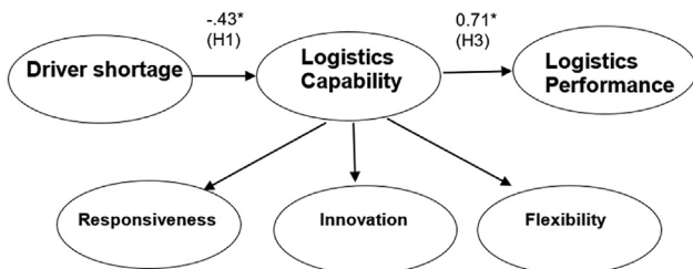
Figure 2. Path model. Note: *p-value <.001.
