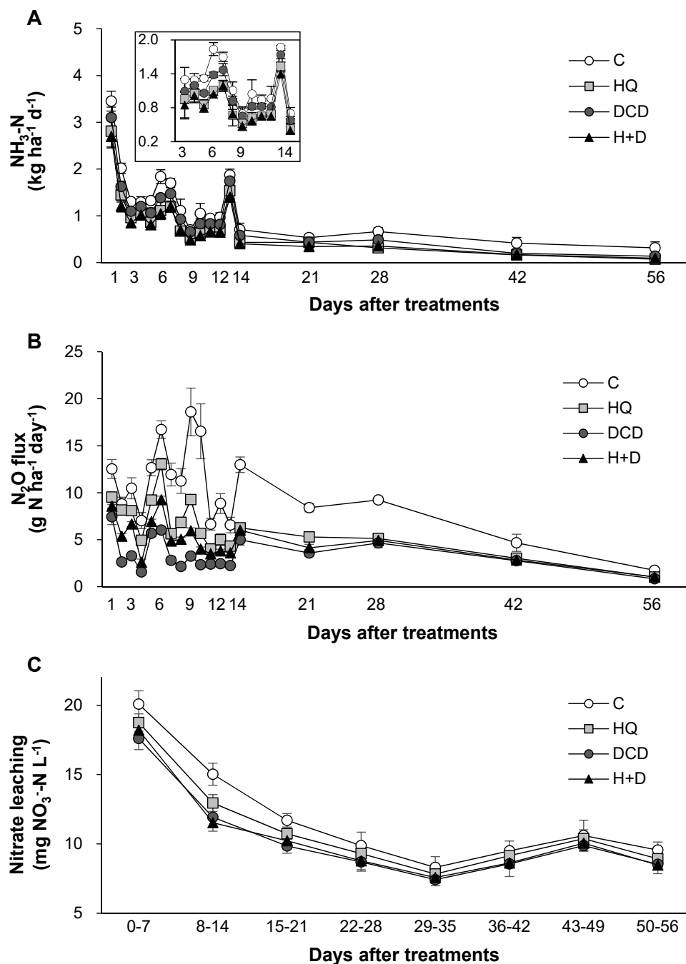
Figure 4. Daily emissions of ammonia (A) and nitrous oxide (B) and weekly accumulative nitrate concentration in leachate (C) from the control (○), urease inhibitor (HQ, ◻), nitrification inhibitor (DCD, ●) and the combination of HQ and DCD (H+D, ▲) during regrowth of perennial ryegrass sward. HQ, hydroquinone; DCD, dicyandiamide.
