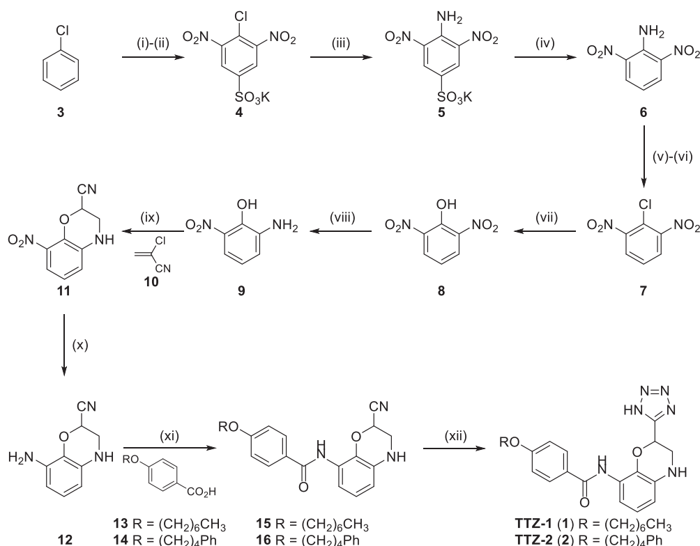
Figure 7. Synthesis of TTZ-1 (1) and TTZ-2 (2). Reagents and conditions: (i) H 2 SO 4 (conc), 120 °C, 4 h. (ii) H 2 SO 4 (conc):H 2 O (1:1), Δ, 16 °C (36%, four steps). (v) NaNO 2 , H 2 SO 4 , 40 °C, 1 h. (vi) CuCl, HCl(conc), 80 °C, 20 min (57%, two steps). (vii) KOH, H 2 O, Δ, 1 h (quant). (viii) 10% Pd/C, H 2 , MeOH, r.t., 1 h (88%). (ix) 10 (8.0 equiv.), Cs 2 CO 3 , PhMe, Δ, 4 h (15%). (x) 10% Pd/C, H 2 , MeOH, r.t., 1 h (70%). (xi) 13 (1 equiv.) or 14 (1 equiv.), HATU, DIPEA, DMF, r.t., 16 h ( 15 58%; 16 45%). (xii) NaN 3 , NEt 3 -HCl, DMF, 140 °C, 2 h ( 1 quant; 2 quant). TTZ, tetrazole.
