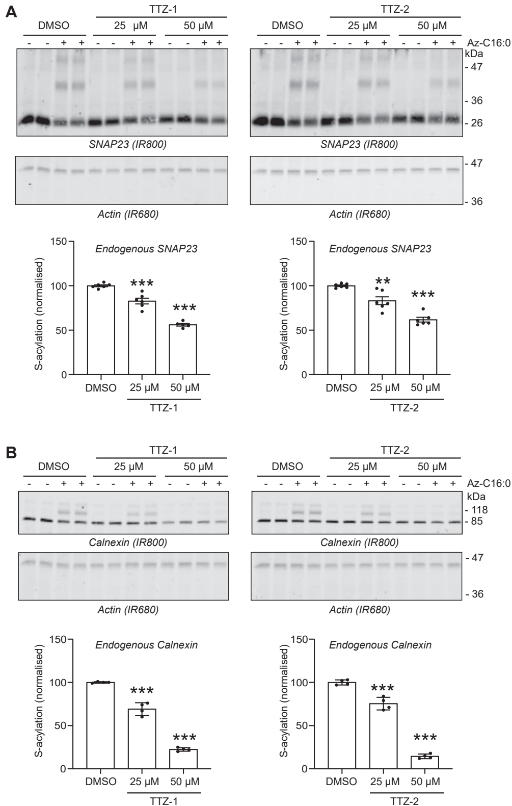
Figure 10. Activity of TTZ-1 and TTZ-2 against the S-acylation of endogenous proteins in mammalian cells. HEK293T cells were preincubated for 4 h with TTZ-1 or TTZ-2 (25 or 50 μM final) or DMSO control before metabolic labeling with 100 μM of either palmitic acid (–Az-C16:0) (as a control) or C16:0-azide (+Az-C16:0) for 4 h. Cells were lysed, and proteins having incorporated C16:0-azide were labeled by click chemistry with an alkyne-mPEG5K. Protein samples were then resolved by SDS-PAGE and transferred to nitrocellulose membranes that were first probed with either an anti-SNAP23 antibody (A) (IR800) or an anti-calnexin antibody (B) (IR800) and then probed with an anti-actin antibody (IR680). Representative images are shown. Positions of the molecular mass markers (in kilodalton) are indicated on the right side of the membranes. Two (A) or three (B) independent experiments were performed in duplicate. The data were quantified, and the graphs below each set of membranes show mean ± SEM of normalized S-acylation of either endogenous SNAP23 (A) or endogenous calnexin (B). Filled circles represent individual samples. Statistical analysis (ANOVA) was performed to reveal whether there was a significant difference between the substrate S-acylation of cells treated with DMSO versus similar samples treated with TTZ-1 or TTZ-2 (** p < 0.001; *** p < 0.01). DMSO, dimethyl sulfoxide; HEK293T, human embryonic kidney 293T cell line; TTZ, tetrazole.
