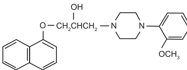
Figure 1 Chemical structure of naftopidil (C 24 H 28 N 2 O 3 ), molecular weight 392.5.
