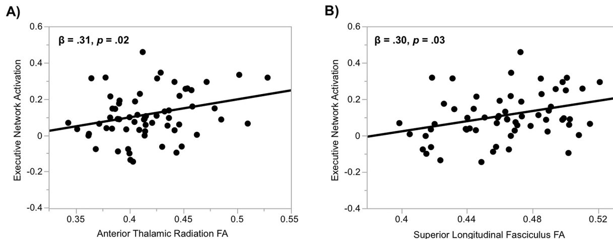
Fig. 3. Scatter plot with line of best fit illustrating positive associations between n -back executive network activation and bilateral gait-associated FA in the (A) anterior thalamic radiation and (B) superior longitudinal fasciculus.
