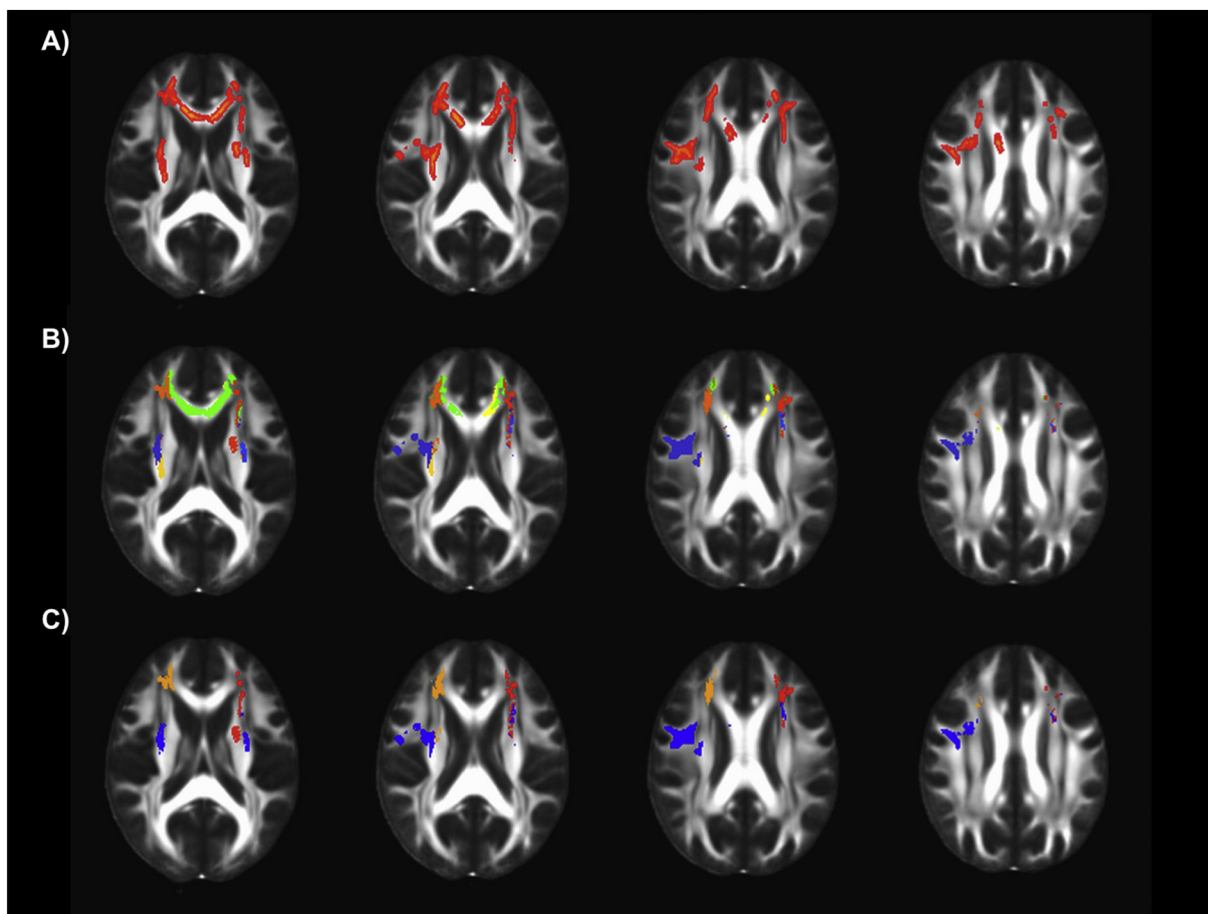
Fig. 2. Regional FA associations with walking speed (A) adjusted for all covariates and corrected to p < 0.05 , (B) broken into JHU tracts (ref. Table 2), and (C) found to be significantly associated with activation after adjusting for scanner, age, and sex. Voxels surviving adjustment were located in the left and right anterior thalamic radiation (red/yellow), and the right superior longitudinal fasciculus (blues). (Left = Right).
