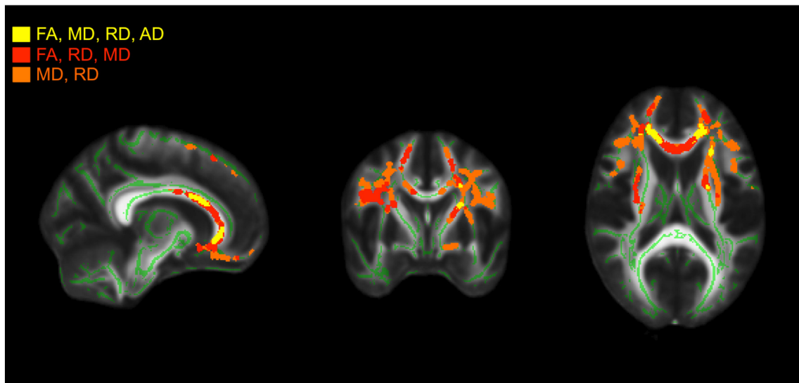
Fig. 1. Regions of white matter showing a significant relationship (corrected p < .05 ) between walking speed and diffusion parameters, such that participants exhibiting greater white matter integrity (i.e., higher FA, lower AD, RD, and MD) walked faster. (Left = Right).
