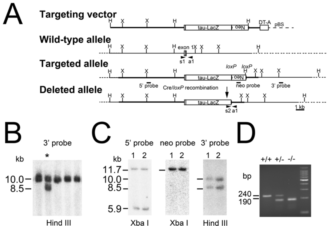
Fig 3. Generation of OCAM-deficient mice. (A): Gene targeting strategy to generate OCAM-deficient mice. The pgk-neo gene (Neo) flanked by loxP site and tau-lacZ gene (tau-LacZ) was inserted into the first exon of OCAM gene. H, Hind III; X, Xba I; pBS, pBluescript II. (B): Southern blot analysis of ES clones. ES cell DNA was digested with Hind III and hybridized with OCAM-3' probe indicated in (A). The homologous recombinant clone is indicated with asterisk (*). (C): The correct integration of the targeting vector was confirmed by Southern blotting of Hind III or Xba I digest with probes indicated in (A) on two of positive clones. (D): PCR genotyping of WT (wild-type, +/+), heterozygous (+/-), and homozygous KO (knock out, -/-) OCAM mutant mice. The primer specific to each allele (s1–s2, a1) were indicated.
