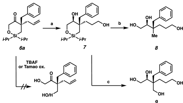
Scheme 3 Synthesis of highly oxygenated, chiral, acyclic quaternary stereocenters: (a) \text{BH}_3 \cdot \text{SMe}_2 , THF, 23 °C, 18 h; \text{H}_2\text{O} , 23 °C, 10 min; \text{NaBO}_3 \cdot 4\text{H}_2\text{O} , 23 °C, 4 h, 58% yield, dr = 93 : 7; (b) TBAF, DMF, 80 °C, 18 h, 77% yield; (c) TBAF, \text{NaBO}_3 \cdot 4\text{H}_2\text{O} , THF, 60 °C, 18 h, 51% yield.
