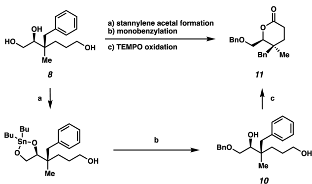
Scheme 4 Synthesis of lactone bearing vicinal quaternary-trisubstituted stereocenters: (a) \text{Bu}_2\text{SnO} , MeOH, reflux, 18 h; (b) BnBr, TBAF, toluene, reflux, 20 h, 60% yield over 2 steps; (c) TEMPO, PIDA, \text{CH}_2\text{Cl}_2 , 23 °C, 18 h, 65% yield.
