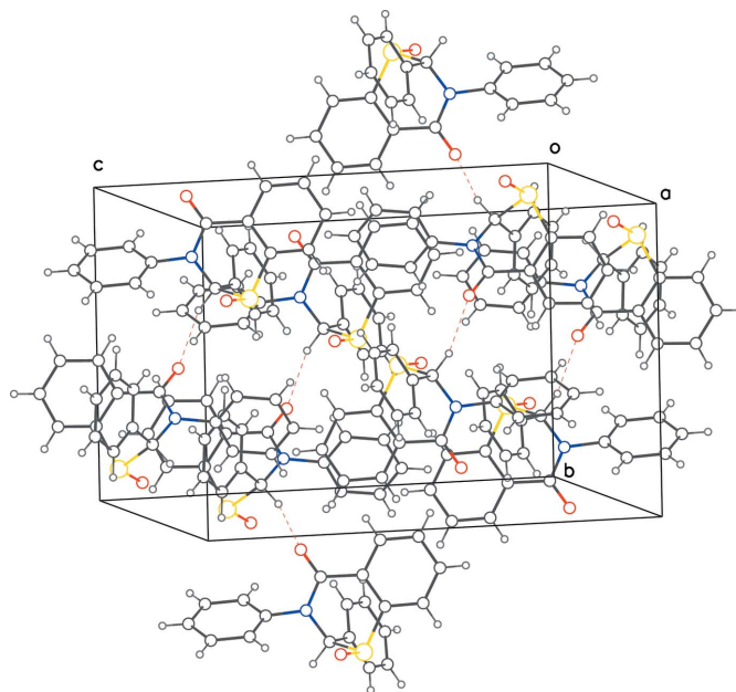
Figure 2 Crystal packing diagram showing C-H\cdots O contacts as dotted red lines between molecules of (I) which form chains along the b -axis direction.
