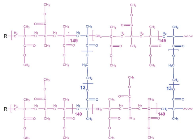
Fig. 1 PGPE chemical structure, C=O groups on backbone and EO groups on crosslinker.
