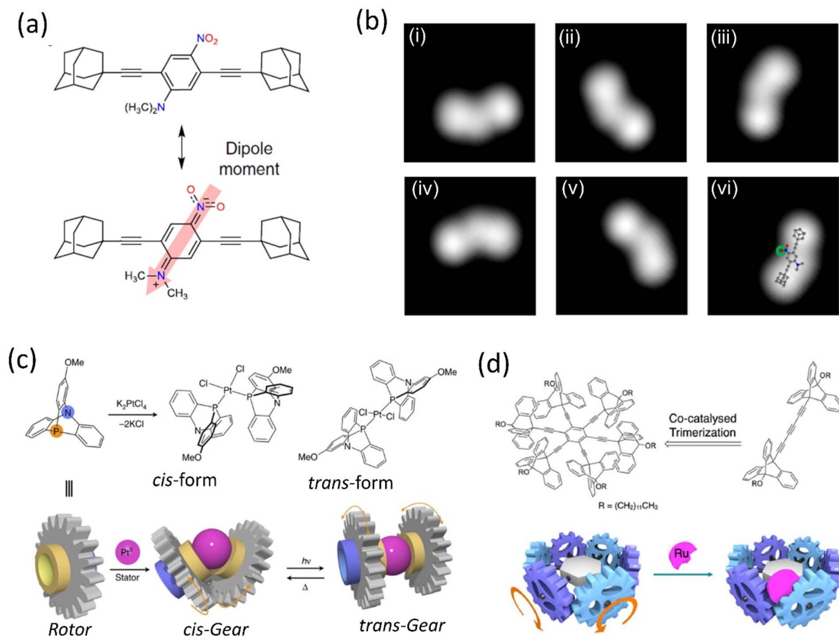
Fig. 7 (a) Chemical structure of polar motor. (b) (i)–(vi) STM images of the molecule showing clockwise rotation upon applied voltage pulse. Reproduced with permission. 130 Copyright 2019, The Authors, published by Springer Nature. (c) Schematic representation of a Pt II -centered molecular gear exhibiting cis – trans isomers could be achieved upon ultraviolet irradiation at 360 nm and heating. Reproduced with permission. 134 Copyright 2017, The Authors, published by Springer nature. (d) Ru-centered sextupled triptycene gear. Reproduced with permission. 135 Copyright 2017, American Chemical Society.
