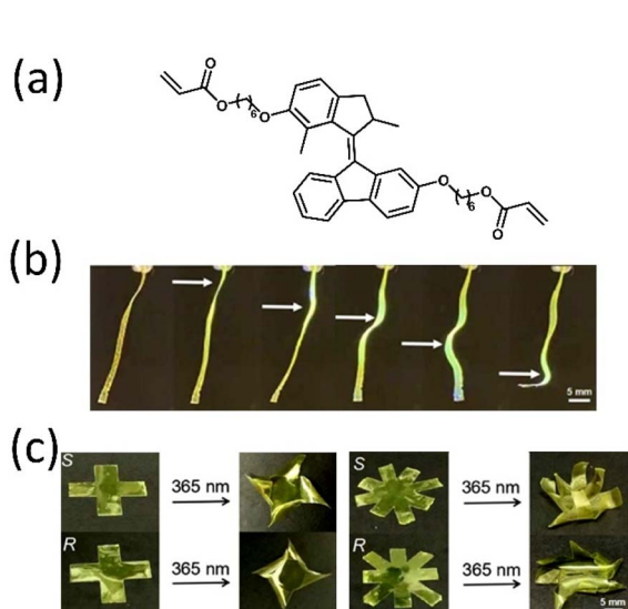
Fig. 21 (a) Molecular structure of a rotary motor. Light-powered (b) wavy motion and (c) helical motion of the motorized LC film (scale bar is 5.0 mm). Reproduced with permission. 200 Copyright 2022, The Authors, published by American Chemical Society.
