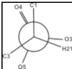
Fig. 2. Newman projection along the C2—P bond.
