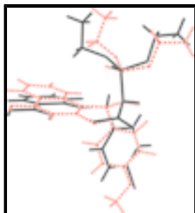
Fig. 3. A superposition of structures (I) and (II). The latter is indicated in the dashed line. The least-squares fit was based on all common non-H atoms of the 3,4-dihydrocoumarin moiety; the r.m.s. deviation was 0.10 Å.
