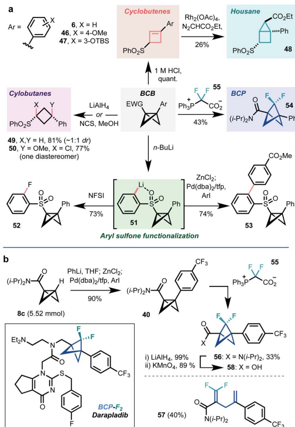
Scheme 2 (a) Further transformations of 1,3-disubstituted BCBs. (b) Application to synthesis of the BCP-F 2 -darapladib sidechain.
