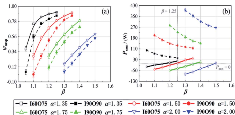
Fig. 22 The experimental results regarding (a) the static pressure increase ratio \psi_{\text{msp}} and (b) the gas loading power consumption P_{\text{con}} .
