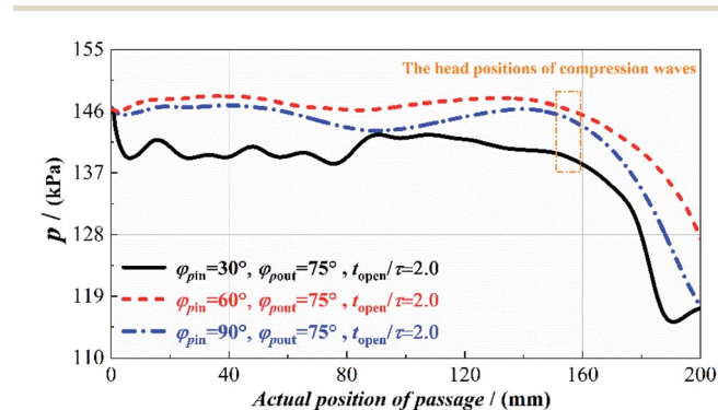
Fig. 15 A comparison of pressure distributions along the channels.
