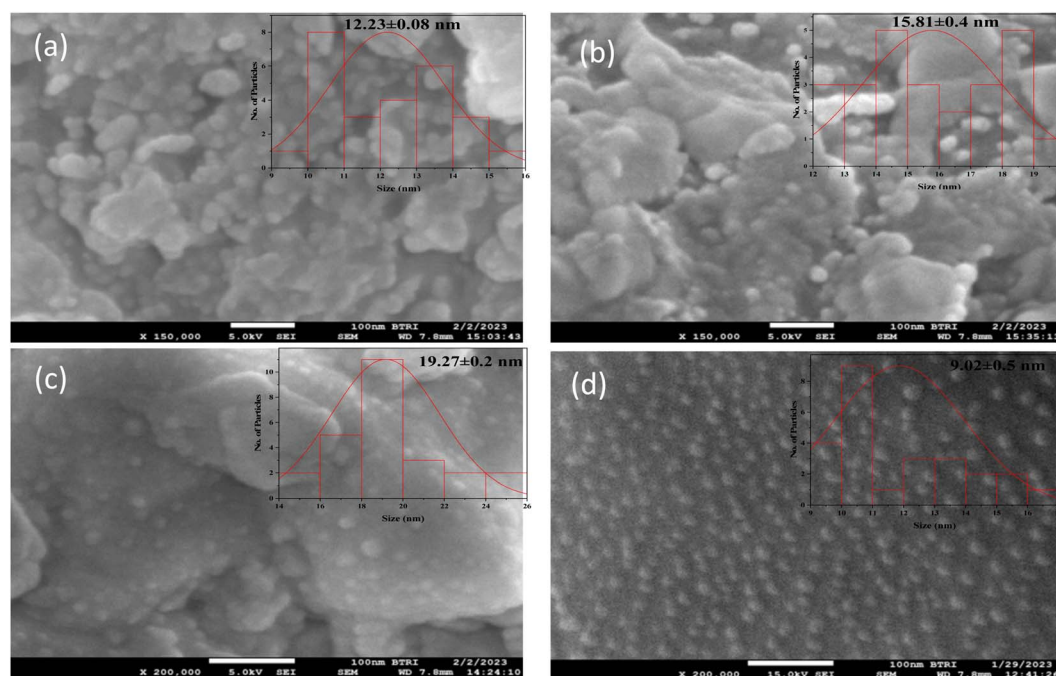
Fig. 5 FE-SEM images with grain size distribution of AgNPs for (a) 10 mM (b) 15 mM (c) 20 mM and (d) 25 mM of AgNO 3 solution.
