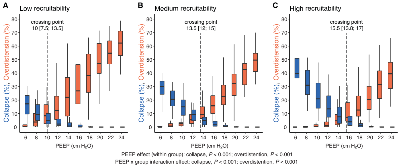
Figure 3. Distribution of collapse (blue) and overdistension (orange) during the decremental positive end-expiratory pressure (PEEP) trial for the three groups of recruitability (A: low recruitability, B: medium recruitability, C: high recruitability). The dotted lines indicate the group median [interquartile range] PEEP level as per the crossing point of the collapse and overdistension curves.
