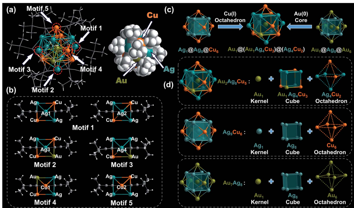
Fig. 3 Structural analysis in body-centered cubic (BCC) M_{15} NCs. (a) Overall and space-filling structure of monocationic Au_2Ag_8Cu_5 , (b) the five types of linear {}^tBu-C\equiv C-Cu\equiv C-{}^tBu staple motifs on the metal surface. Coordination modes of {}^tBu-C\equiv C ligands: \mu_2-\eta_1 (Ag/Cu), \eta_1 (Ag); \mu_2-\eta_1 (Au/Ag/Cu), \eta_1 (Ag); \mu_2-\eta_1 (Au/Ag/Cu), \eta_1 (Cu) and \mu_2-\eta_1 (Ag/Cu), \eta_1 (Cu). (c) Structural analysis and (d) anatomy of BCC M_{15} kernel in Au_2Ag_8Cu_5 , Ag_9Cu_6 , and Au_7Ag_8 , respectively. Color legend: Au, yellow; Ag, cyan; Cu, orange; C, gray; H, white.
