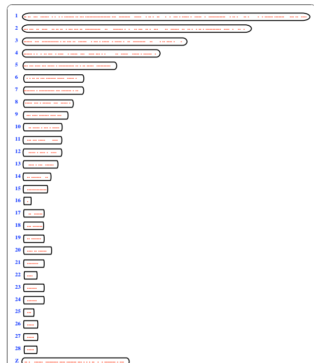
Figure 1 Chromosomal locations of orthologous kiwi genes recovered in this study on the chicken genome.
