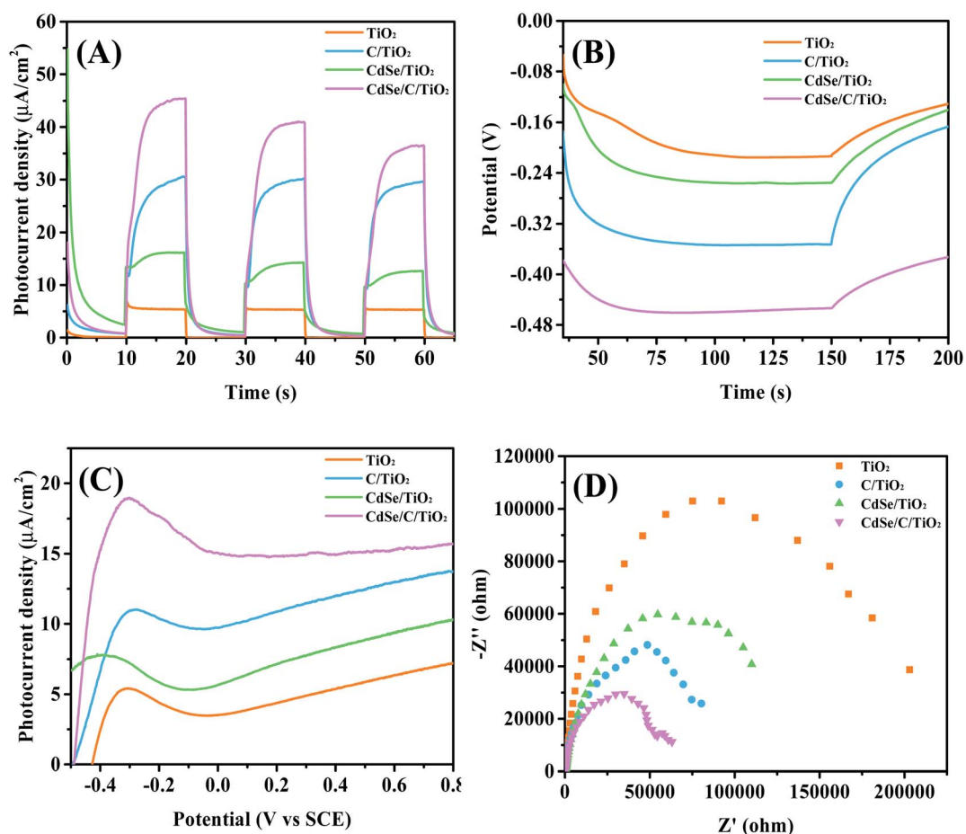
Fig. 6 (A) Transient photocurrent responses; (B) open circuit potential ( versus SCE); (C) linear sweep voltammetry curves; (D) electrochemical impedance spectroscopy for pure \text{TiO}_2 , \text{C/TiO}_2 , \text{CdSe/TiO}_2 and \text{CdSe/C/TiO}_2 nanofilm.
