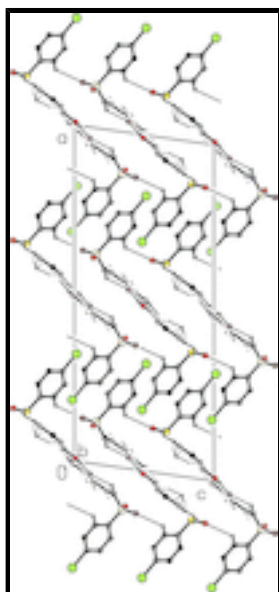
Fig. 3. The molecular packing and hydrogen bonding for (I), viewed down the b axis. Hydrogen atoms not involved in the showed interactions have been omitted for clarity.
