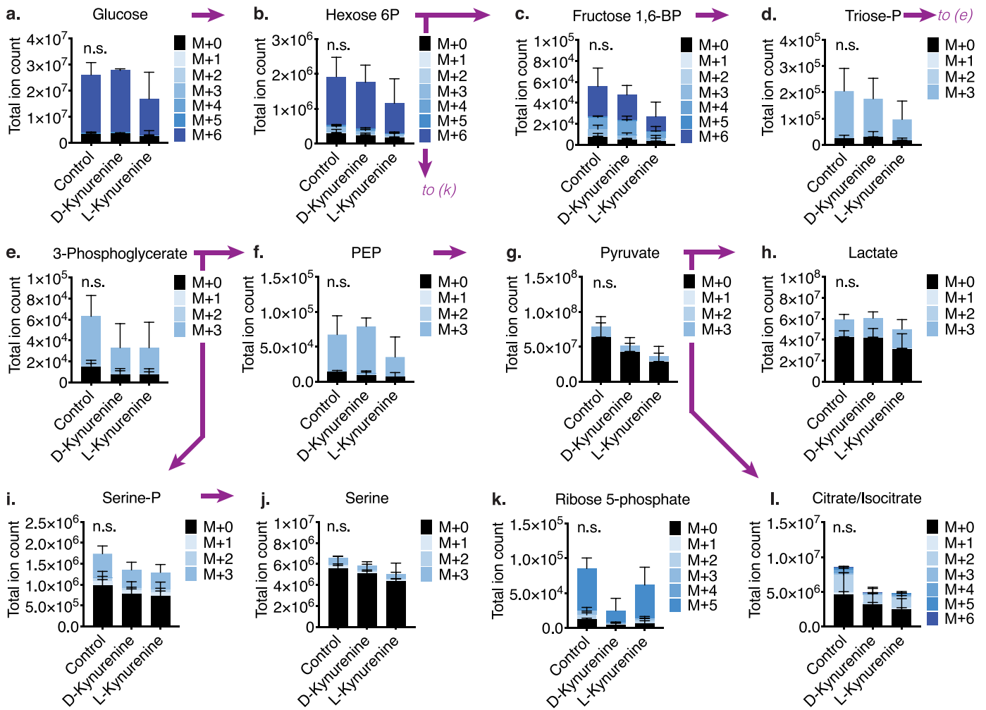
Figure 4. D- and L-kynurenine do not significantly alter glycolytic flux. Tconv were co-stimulated with CD3 \epsilon /CD28 mAb-coated beads for 20 hours and were then cultured with [ ^{13} C _6 ] D-glucose for three hours with either 1 mM of L- or D-kynurenine. Metabolites were extracted and analysed for derivative analysis, with M+1-6 indicating the number of [ ^{13} C]-atoms per isotopologue (3/group, one-way ANOVA). (a-h) Glucose and glucose-derived glycolytic intermediates were not significantly altered by the addition of L- or D-kynurenine. (i-l) Likewise, kynurenine treatment did not alter glucose-derived contributions to serine production (i, j), the pentose phosphate pathway (k), and the Krebs cycle (l). Error bars indicate SEM.
