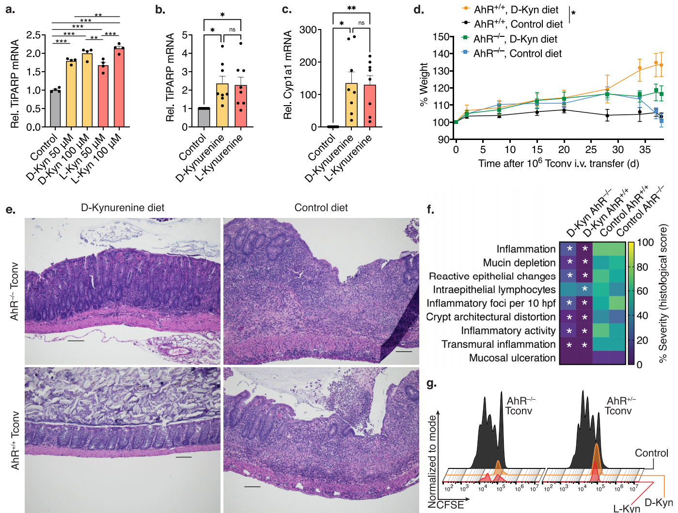
Figure 3. D- and L-Kynurenine activate AhR signalling which mediates part but not all of the immunosuppressive T cell response. (a-c) AhR-dependent gene expression via qPCR. Both D- and L-kynurenine invoke AhR signalling in glioblastoma cells (a) as well as in co-stimulated Tconv (b, c). (a) 3/group, one-way ANOVA (b, c) 8/group, paired Student t-test. (d) B6/Rag1 -/- colitis as in Figure 2D with 10 6 AhR +/+ and AhR -/- adoptively transferred Tconv (5/group, area under the curve, one-way ANOVA). (e, f) Representative tissue sections and blinded colitis histology scoring. (e) Colonic specimens from B6/Rag1 -/- mice after colitis induction via adoptive Tconv transfer. Specimens from mice receiving control rather than D-kynurenine diet show significant colitis. The beneficial effect of D-kynurenine is diminished if the adoptively transferred Tconv lack AhR. Haematoxylin and eosin staining; scale bar 100 \mu m. (f) Heatmap of blinded histological scoring normalized to a percent scale (two-way ANOVA, 5/group, * indicates p < 0.05 relative to control diet and AhR +/+ Tconv cell condition). (g) AhR +/+ and AhR -/- Tconv were CFSE-labelled and co-stimulated with or without 1 mM L- and D-kynurenine for three days. Absence of AhR did not protect T cells from apoptosis. *, **, and *** indicate p < 0.05, p < 0.01, and p < 0.001, respectively. Error bars indicate SEM.
