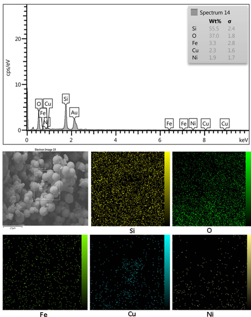
Fig. 6 EDS of \text{NiFe}_2\text{O}_4@/\text{SiO}_2\text{-Cu} and elemental mapping of Fe, Ni, O, Si, Cu.
