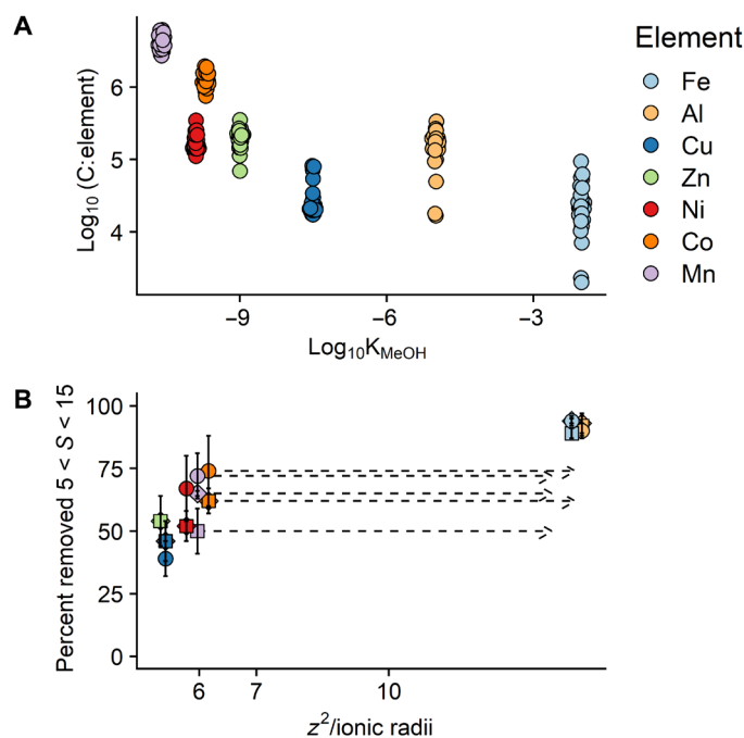
Fig. 6. Influence of chemical periodicity on TM SPE-DOM biogeochemistry in the Amazon estuary. (A) The decrease in C:TM ratios (circles show log 10 values for the MMW fraction as a quasi-random density plot) is consistent with trends in other thermodynamic stability constants of metal complexes as illustrated here for first hydrolysis constant (log 10 K MeOH ). Cu, Co, and Mn were assumed to be present in the +2 oxidation state, while Fe was assumed to be in the +3 oxidation state. (B) The proportion of TM SPE-amb fraction that is removed at low salinity increased with polarizing power of the TM ion as expressed by the square of the oxidation state ( z^2 ) divided by Shannon's ionic radii. Diamond symbols show the percentage removed for the total TM SPE-amb concentrations determined by SEC, squares removal of the MMW fraction, and circles removal of the Hphob fraction. For Mn and Co, the dashed arrow represents the increase in polarizing power that results from oxidation from the +2 oxidation state to the +3 oxidation state. Note the log 10 scale for polarizing power.
