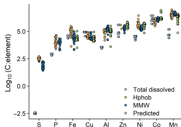
Fig. 5. Elemental stoichiometry observed in MMW and Hphob fractions. Elements are ranked on the x axis according to their stoichiometry in the MMW fraction. C:element ratios are plotted as log 10 values using a quasi-random density plot. “Total dissolved” points show the ratio calculated for dissolved elements to DOC using concentrations of S as sulphate (calculated from salinity), DIP, and total dissolved TM concentrations. Predicted values were obtained from calculations of TM speciation at ambient salinity, pH, and dissolved TM and DOC concentrations, assuming that binding sites in DOM scale to DOC. We assumed that TM-DOM binding could be represented by the NICA model combined with the Donnan model for electrostatic interactions. For calculations of C:Fe ratios, we assumed competition between NICA binding sites and the formation of Fe(OH) 3 (s) (19).
