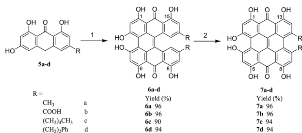
Scheme 1 General synthetic pathway of hypericin ( 7a ) and its derivatives ( 7b–d ). Reagents and conditions: (1) 1.5% NaOH/H 2 O, pyridine- N -oxide, FeSO 4 ·7H 2 O, 105 °C, 10 W, 70 min, N 2 by microwave reactor; (2) 575 nm monochromatic light, acetone, N 2 , 60 min.
