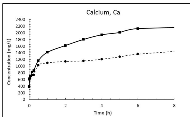
Figure 8. Concentration of calcium in sea water at T = 5 °C (dashed line) and 15 °C (solid line) as function of time after adding 1% (w/v) fine CaO.
