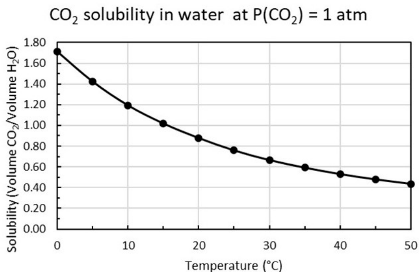
Figure 4. Dissolved CO 2 versus temperature (°C) for carbon dioxide pressure P(\text{CO}_2) = 1 atm plotted from tabular data [14].
