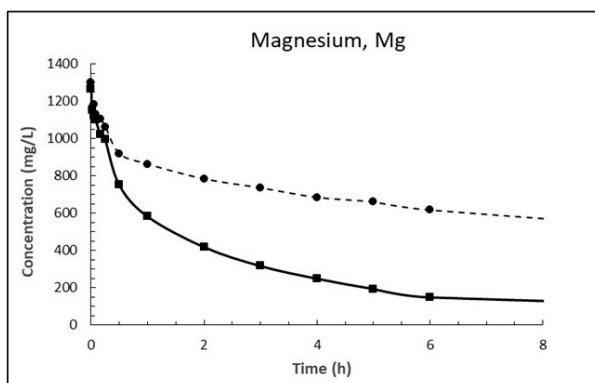
Figure 7. Concentration of magnesium in sea water at T = 5 °C (dashed line) and 15 °C (solid line) as function of time after adding 1% (w/v) fine CaO.
