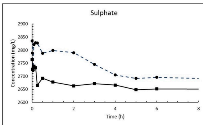
Figure 9. Concentration of sulphate in sea water at T = 5 °C (dashed line) and 15 °C (solid line) as function of time after adding 1% (w/v) fine CaO.
