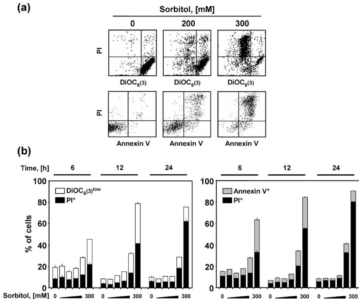
Fig. 1 Hyperosmotic stress-induced apoptosis in HeLa cells. HeLa cells were treated for up to 24 h with 0 (control), 25, 50, 100, 200 or 300 mM sorbitol, then submitted to cytofluorometric analysis of mitochondrial membrane potential (DiOC 6 (3) staining), PS exposure (Annexin V staining) and viability (PI staining). (a) Representative dot plots of HeLa cells treated for 24 h with 0, 200 and 300 mM sorbitol. X-axis, DiOC 6 (3) (upper panels) and Annexin V staining (lower panels); Y-axis, PI staining. (b) Time- and dose-dependent response of HeLa cells to sorbitol. White columns depict the percentage of cells that have a low mitochondrial membrane potential but are still viable (DiOC 6 (3) low ). Black columns report the percentage of cells that have lost the intactness of plasma membrane (PI + ). Light grey columns indicate the percentage of cells that have exposed PS on the outer leaflet of the plasma membrane (Annexin V + ). Data are mean of triplicate experiments \pm SEM. (c) ROS generation. HeLa cells were treated with 300 mM sorbitol
