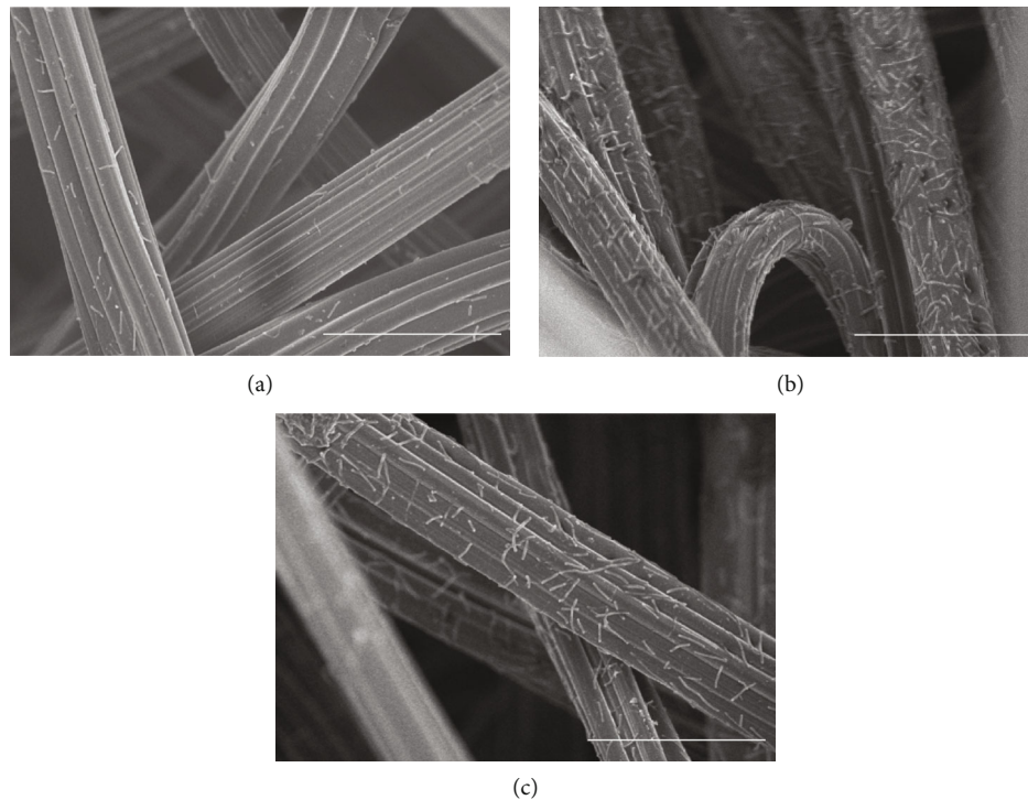
FIGURE 4: SEM images of carbon felt: (a) distilled water (control), (b) NaOH, and (c) HCl treated. Scale bar = 30 \mu\text{m} .
