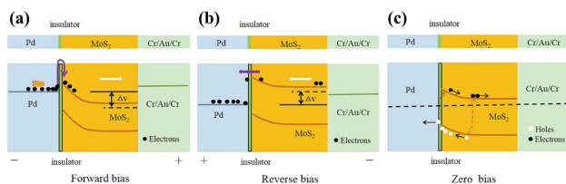
Fig. 6 The energy band diagrams of the fabricated MIS structured photodetectors. The energy band diagram of the MIS structured photodetectors (a) with a forward bias (the purple arrow is the tunneling current. The black dash dot line is the Fermi level at thermal equilibrium), (b) with a reverse bias (the purple arrow shows thermionic emission of electrons), and (c) at zero bias, respectively.
