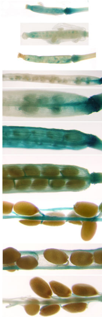
AtbZIP44
