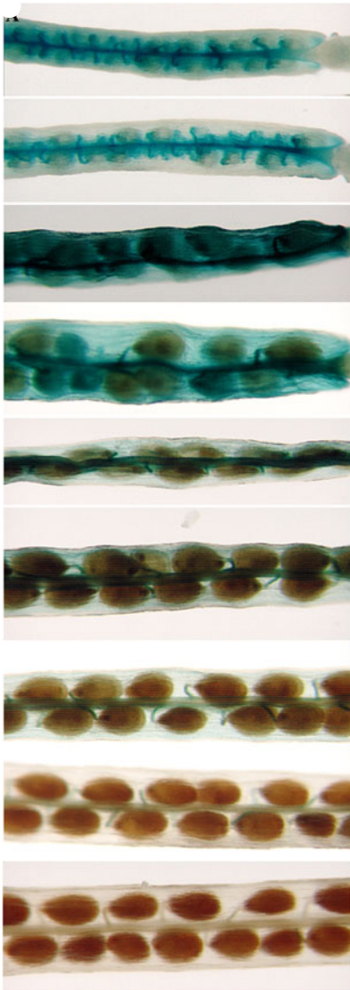
AtbZIP11 /ATB2
