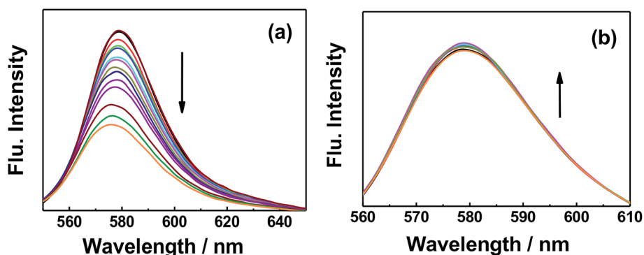
Fig. 10 Fluorescence changes of RhB ( 1.7 \times 10^{-5} M) with the addition of different concentrations of (a) GO and (b) GO-Fe 3 O 4 @ZrO 2 in water.
