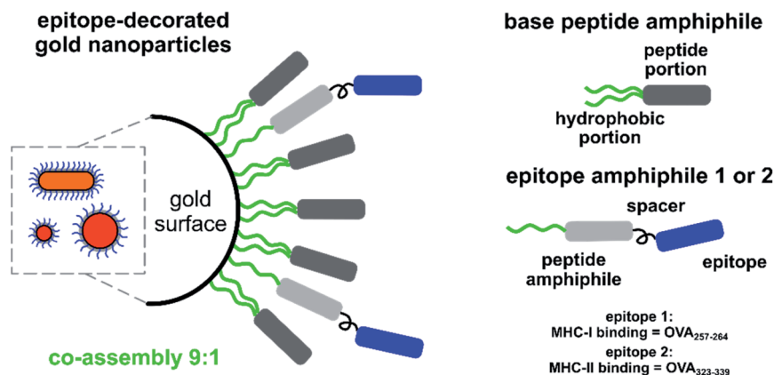
Scheme 1 Schematic representation of the shell composition ( base and epitope-bound peptide amphiphiles 1 and 2 ) used to stabilise GNPs and GNRs. Base was mixed with either 1 or 2 at a 9 : 1 molar ratio to form shells around different GNPs and to provide near-identical surface chemistries.
