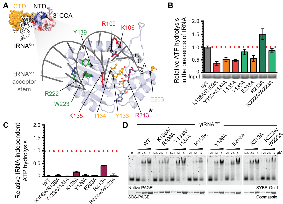
Figure 4. Analysis of tRNA Sec interaction with CtKti12 NTD . (A) (Top left): Structural model of tRNA-bound CtKti12 NTD based on superimposition with MjpPSTK NTD (3ADB), r.m.s.d. = 3.8 Å 2 . tRNA Sec is shown in grey and MjpPSTK CTD in yellow. The 3' end of the superimposed tRNA Sec reaches to the active site of CtKti12 NTD . Surface charge distribution of CtKti12 NTD is shown in blue and red. Positively charged regions (blue) coincide with a modelled contact surface with tRNA Sec . Color coding and scale are identical to Figure S5. (Bottom right): The close up of the model shows the proposed tRNA interaction surface at the NTD, which is shown in light blue, acceptor stem of tRNA Sec is gray. Mutants with significantly downregulated ATPase activity are shown in red, mutants with moderate ATPase properties in orange. Hydrolytic activity after mutating residues shown in green does not differ significantly from WT protein. The gatekeeping R213 residue (asterisk) is shown in violet. (B) Analyses of hydrolytic properties of tRNA interaction surface mutants using the malachite green assay. Calculated standard deviations are shown ( n = 3 ). Color coding as in (A). (C) tRNA-independent ATP hydrolysis of mutants within tRNA-interaction interface on the NTD using the malachite green assay. The results were normalized to the tRNA Sec -induced hydrolysis of WT protein and calculated standard deviations are shown ( n = 3 ). (D) Binding affinity of tRNA-interface mutants to the bulk yeast tRNA. Samples were resolved on a 5% native PAGE. As a loading control, samples were also analyzed by denaturing SDS-PAGE stained with Coomassie. tRNA was stained using SYBR-Gold.
