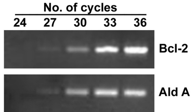
Fig. 2: Determination of the exponential range of amplification for Bcl-2 and Aldolase A. The analysis was performed in 1 mM MgCl 2 at 65°C. The intensity of the Bcl-2 amplification product increased up to 36 cycles, whereas Aldolase A(Ald A) reached a plateau at 33 cycles.
