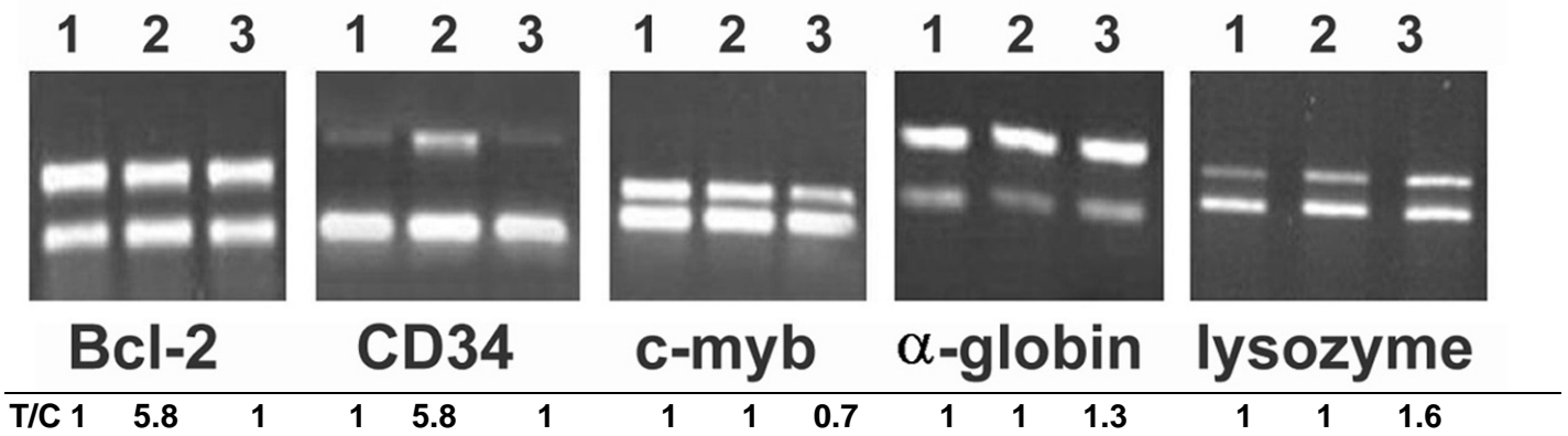
Fig. 4: Example of analyses performed on different target RNAs in the same set of samples: effect of TGF- \beta 1 on TF-1 cells. Lane 1 is control TF-1 cells, lane 2 treatment with TGF- \beta 1, lane 3 treatment with anti-TGF- \beta 1. In all panels, the upper band is the target and the lower band is the amplification product of Aldolase A. T/C indicates the relative level of the target amplification product (T) over the Aldolase A internal control (C) after normalization to the control sample, i.e. it expresses the change in folds with respect to the untreated control (lane 1).
