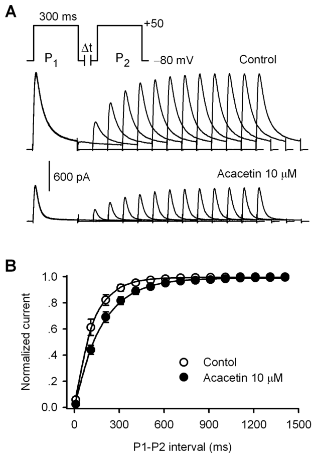
Figure 4. Effect of acacetin on recovery of hKv4.3 current from inactivation. A. Protocol and hKv4.3 current traces recorded in a representative cell before (control) and after 10 \mu M acacetin (8 min) used to assess the time constant of recovery of the channel from inactivation. B. Mean values of recovery time course of hKv4.3 current from inactivation were fitted to a mono-exponential function before and after application of 10 \mu M acacetin. doi:10.1371/journal.pone.0057864.g004
