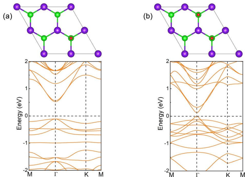
Fig. 2 Top view and calculated band structure of the oxygen functionalized InSe. (a) \text{InSeO}_{0.25} , and (b) \text{InSeO}_{0.5} . The blue, green and red balls represent In, Se and O atoms respectively.
