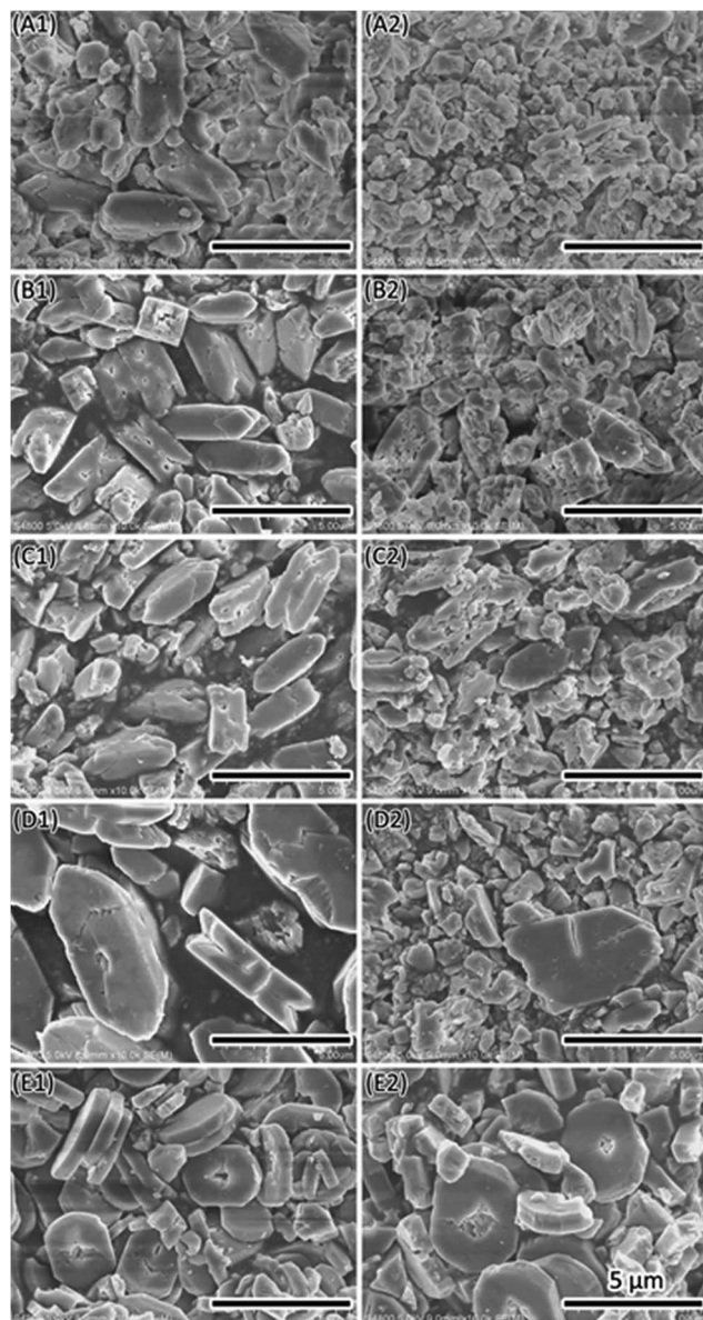
Fig. 3 SEM images show the change of CaO x crystallization time from 0.5 day to 3 days. (A) CaO x , (B) CaO x with D-aspartic acid, (C) CaO x with L-aspartic acid, (D) CaO x with Mg 2+ , (E) CaO x with Na 3 Citrate. 1 to 2 refers to 0.5 day and 3 days, separately.
