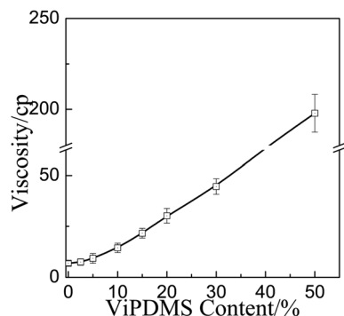
Fig. 2 Viscosity of pigment/monomer dispersion with different ViPDMS content.
