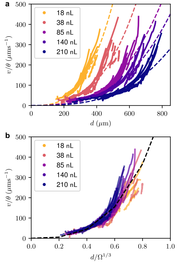
Fig. 4. a) Plot of speed normalized by angle as a function of the distance spanned by droplets for several different volumes. The data for each volume represent 10–15 separate angle experiments. Droplet volume is calculated by taking a volume of revolution of the droplet while symmetric on a single fiber. b) Plot of speed normalized by angle in radians as a function of the aspect ratio of the droplet for a series of volumes.
