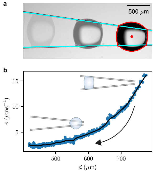
Fig. 2. a) Image showing three snapshots of the droplet through time ( t = 0, 35, 98 s). The droplet moves from left to right toward the apex. The blue lines (lines going through the fibers) show position tracking for the fibers, the red line (line along the perimeter of the droplet) shows the edge of the droplet, and the central red dot the position of the droplet. The position is defined by the averaged location of all pixels within the red line. b) Plot of droplet speed as a function of the distance between the fibers at the position of the droplet center. We note that the droplet moves toward the apex, thus from the right (large d ) to left (small d ) in this plot (sketches of typical configurations are inset).
