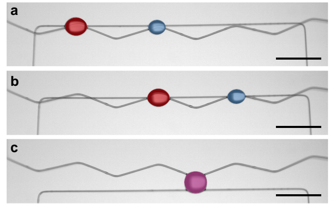
Fig. 6. Series of images showing the use of a sawtooth pattern to first move droplets the same distance and then merge the droplets ( Movie S5 ). The colors are guides to the eye to identify the left and right droplets. a) Initial location of droplets. b) Droplets are moved across one of the teeth in the sawtooth pattern, t = 55\ \text{s} . c) The two droplets are merged, t = 70\ \text{s} . All scalebars are 500\ \mu\text{m} . Larger motions result in simultaneous motion where smaller motions allow for a merger. A detailed mechanism is outlined in Fig. S4 .
