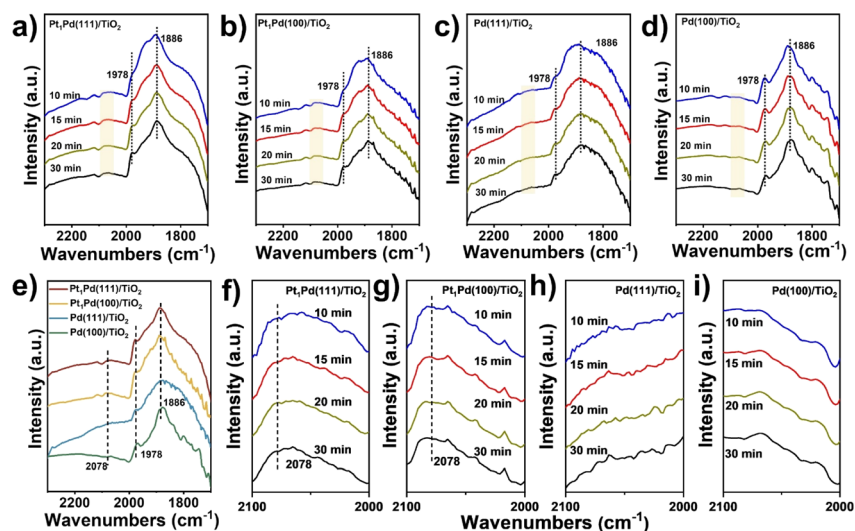
Fig. 3 DRIFT spectra of CO adsorption on (a) Pt 1 Pd(111)/TiO 2 , (b) Pt 1 Pd(100)/TiO 2 , (c) Pd(111)/TiO 2 and (d) Pd(100)/TiO 2 at room temperature at different time points. (e) Comparison of CO-DRIFT spectra at 30 min. (f–i) Magnified CO-DRIFT spectra between 2000 and 2100 cm -1 from (a), (b), (c) and (d), respectively.
