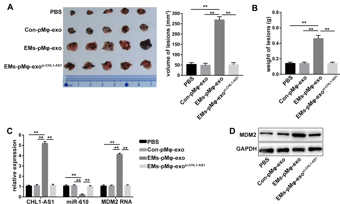
Figure 7 LncRNA CHL1-AS1 in EMs-pM \phi -exo promotes EMs lesions growth by increasing MDM2 in vivo. (A) Total volume of EMs lesions. (B) Total weight of EMs lesions. (C) qRT-PCR was carried out to measure the RNA expression of CHL1-AS1, miR-610, and MDM2 in EMs lesions. (D) MDM2 protein level in EMs lesions was detected by Western blot. **P < 0.01 versus the PBS, Con-pM \phi -exo, and EMs-pM \phi -exo si-CHL1-AS1 groups.
