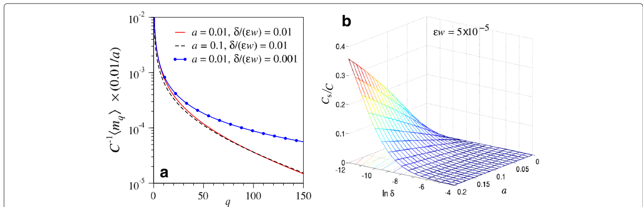
Fig. 5 Clone size distributions and total number of sampled clones. a Expected clone size distributions C^{-1}\langle m_q \rangle derived from the approximation in Additional file 1: Eq. A32 are plotted for various a and \delta/(\varepsilon w) [where w \equiv (1 + \eta)\omega/\mu_d ]. The nearly coincident solid and dashed curves indicate that variations in a mainly scale the distribution by a multiplicative factor. In contrast, the combination \delta/(\varepsilon w) controls the weighting at large clone sizes through the population cut-off imposed by the carrying capacity. Of the two controlling parameters, the steady-state clone size distribution is most sensitive to R \cong \delta/(\varepsilon w) . The dependence of data-fitting on these two parameters is derived in Additional file 1 and discussed in the next section. b For \varepsilon w = 5 \times 10^{-5} , the expected fraction C_s/C of active clones sampled as a function of \ln \delta and a . The expected number of clones sampled increases with carrying capacity K , HSC differentiation rate a = \alpha/r , and the combined sampling and terminal differentiation rate \varepsilon w
