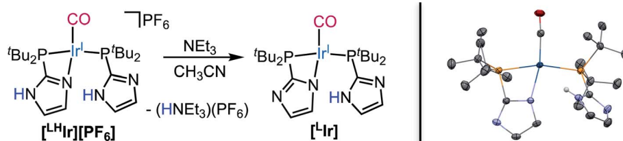
Fig. 4 (Left) Synthesis of [\text{L}^{\text{I}}\text{Ir}] complex by deprotonation of [\text{L}^{\text{H}}\text{Ir}][\text{PF}_6] using \text{NEt}_3 . (Right) Thermal ellipsoid plot of [\text{L}^{\text{I}}\text{Ir}] shown with 50% probability. H-atoms except for N–H and co-crystallized solvent molecules are omitted for clarity.
