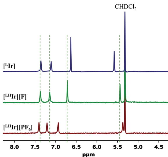
Fig. 5 Partial ^1\text{H} NMR spectra (400 MHz, \text{DCM}-d_2 ) of [\text{L}^{\text{H}}\text{Ir}][\text{PF}_6] , [\text{L}^{\text{H}}\text{Ir}][\text{F}] , and [\text{L}^{\text{I}}\text{Ir}] . Dashed lines are centered at the signals of [\text{L}^{\text{H}}\text{Ir}][\text{F}] .
